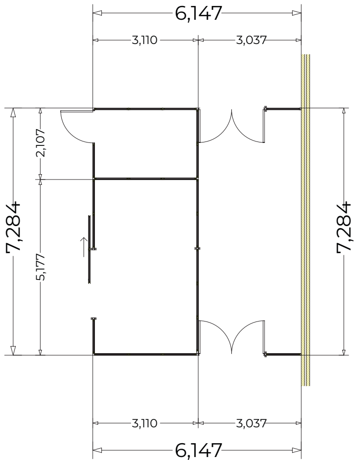
TYPICAL DOUBLESKIN FLOORPLAN LAYOUT
